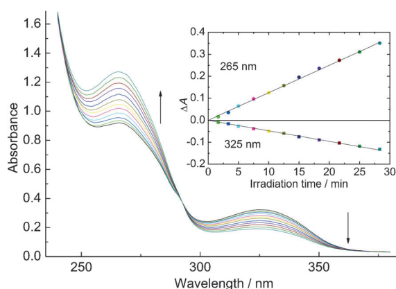
Figure 1. Photorepair of DHT (6-4)PP 10-mer by Xenopus laevis (6-4) photolyase under continuous excitation at 384 nm at 10°C. The solution contained 60 μM DHT (6-4)PP 10-mer, 1.7 μM of photo-reduced (Supporting Information, Section 1 and Figure S7b) XI (6-4) photolyase, 10 mM phosphate buffer at pH 6.8, 100 mM NaCl, 6 mM cysteine, and 5% glycerol in an anaerobic cell. Inset: absorption changes at 265 nm and 325 nm as a function of irradiation time, corresponding to TT restoration and T(6-4)T depletion, respectively. The colors of the symbols correspond to their spectra.
